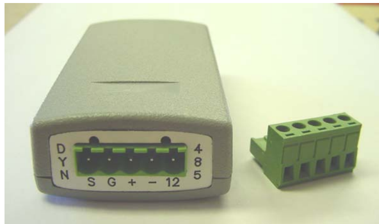
Dynet RS485 Connections
