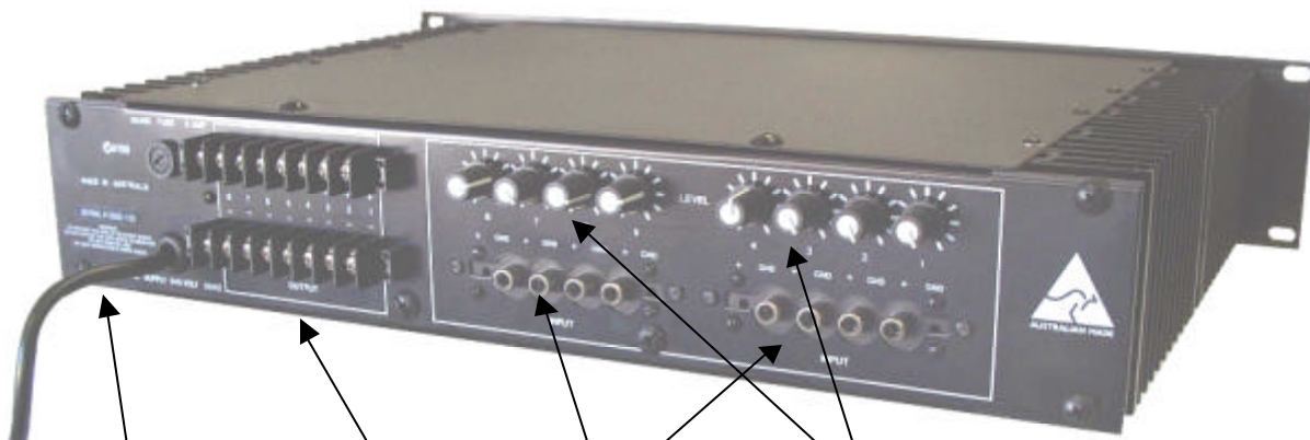
240VAC Supply Speaker Terminations Line Inputs & Input Level Adjustments
